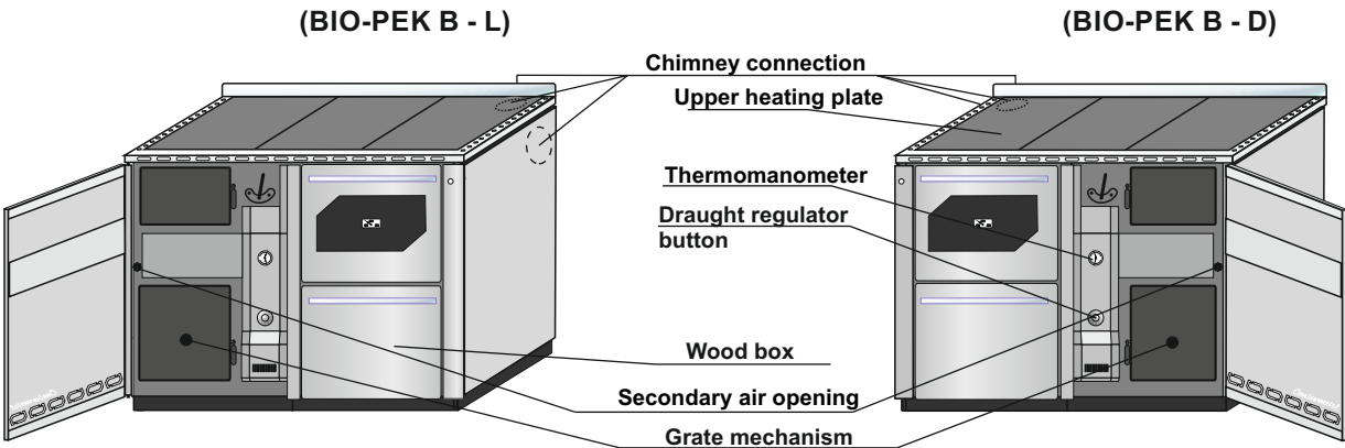
Image 9. Basic parts
